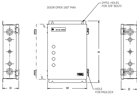
Type 1 enclosure
