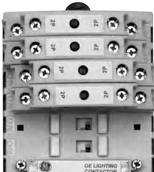
Contactors reconfigured as 4NO-4NC
