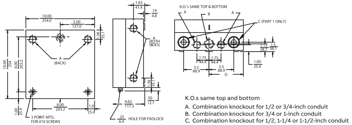
NEMA Type 1 with no CPT, pilot devices or pilot lights, drawing #55-217069 (CR460XE1B)
