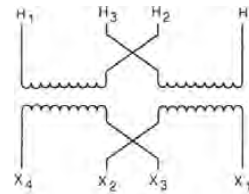
Wiring diagram for low voltage loads
