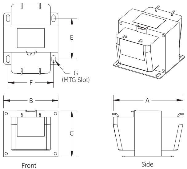
Style AB (Leads Out)
