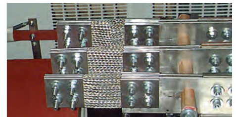
Flexible connectors
