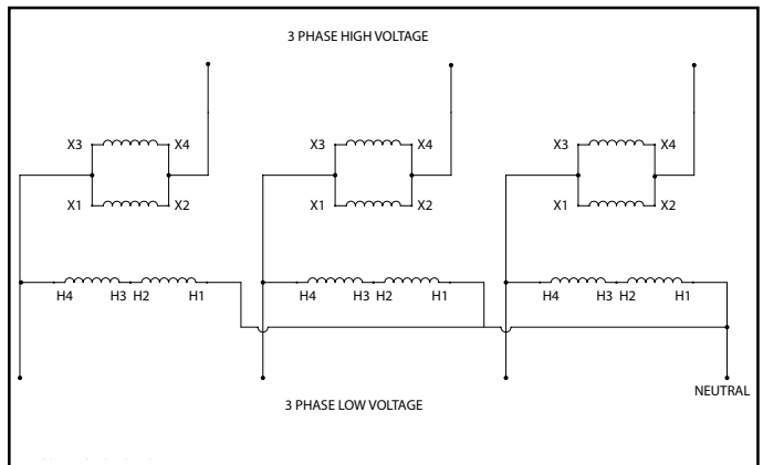
Connection Diagram #12
