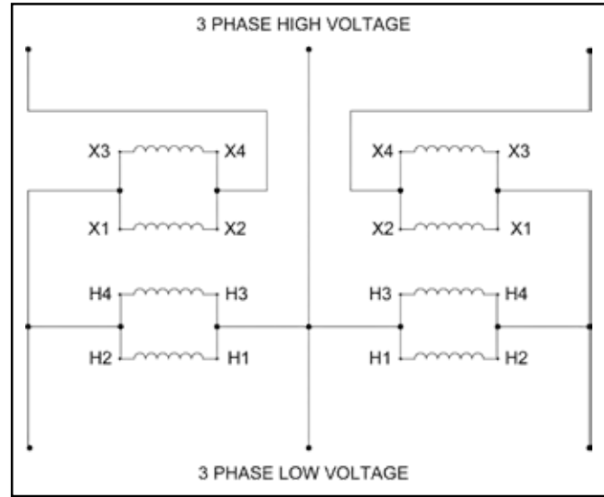
Connection Diagram #6
