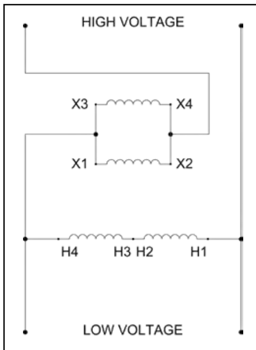
Connection Diagram #3
