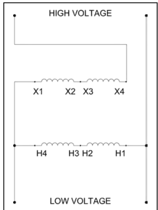
Connection Diagram #4
