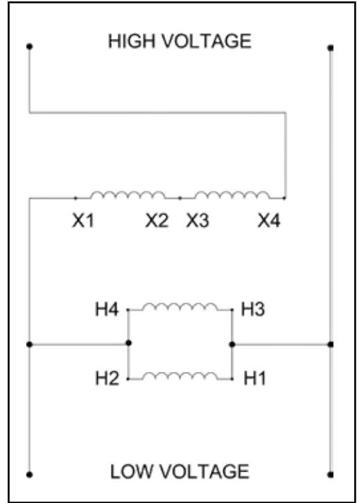
Connection Diagram #2
