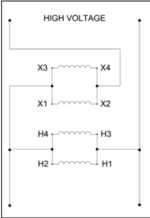
Connection Diagram #1
