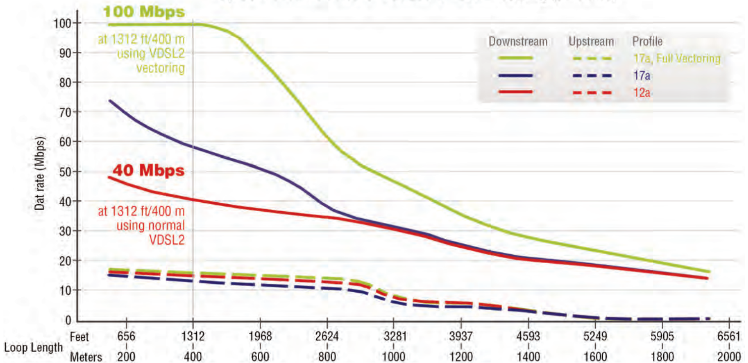
Up/Downstream bitrates for VDSL2 and VDSL2 Vectoring (simulated)
