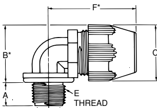
FIGURE 3 (90 DEGREE)
