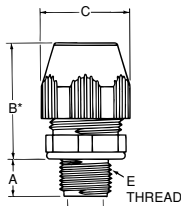
FIGURE 1 (STRAIGHT)
