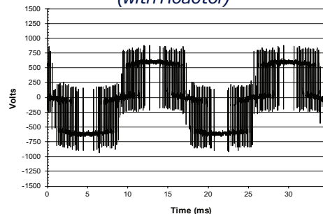
Output Motor Terminal Voltage (with Reactor)
