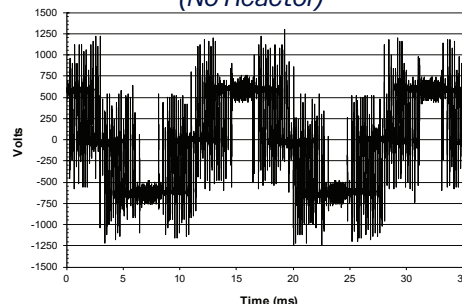
Output Motor Terminal Voltage (No Reactor)
