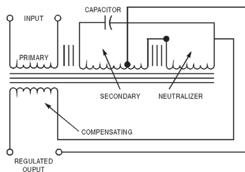
Figure 2: Schematic Diagram
