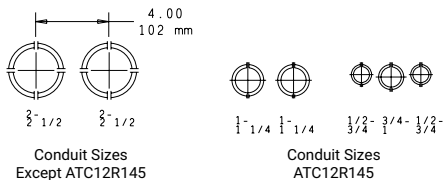
Conduit Sizes all Except ATC12R145 Knockout Pattern (From outside of box)
