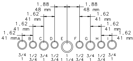
Knockout Pattern
