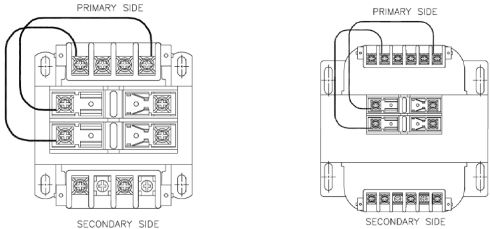
DIAGRAMS BELOW DEPICT NON-SERIES 2 PRIMARY FUSING OPTION
