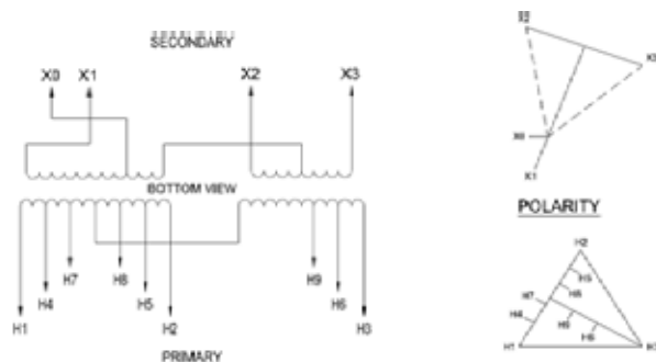
DIAGRAM "280C"
