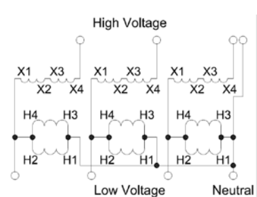
DIAGRAM “N”
