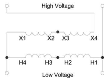
DIAGRAM “F”
