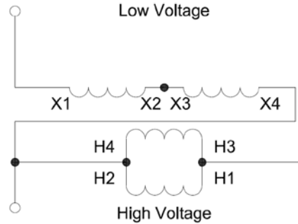
DIAGRAM "D"
