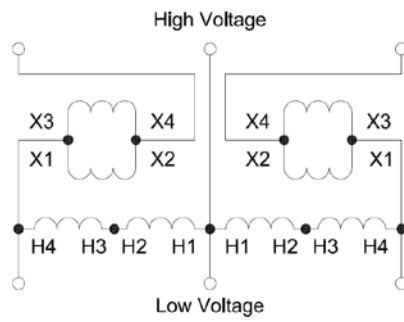
DIAGRAM "I"
