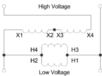
DAIGRAM “B”
