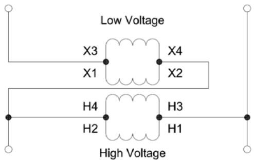
DIAGRAM "C"
