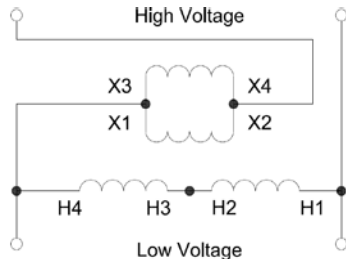
DIAGRAM “E”
