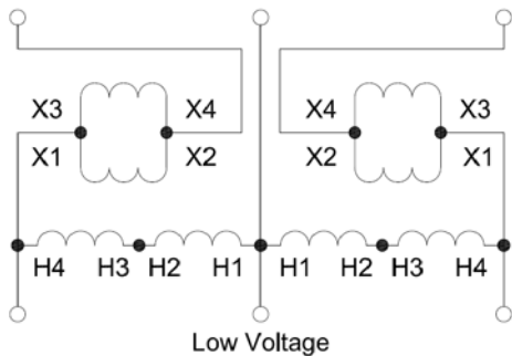
DIAGRAM "M"
