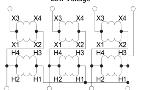
DIAGRAM "O"
