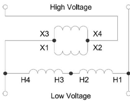
DIAGRAM "E"
