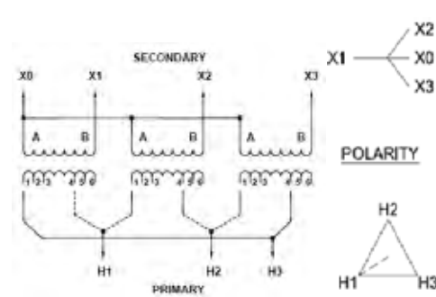
DIAGRAM "DD"
