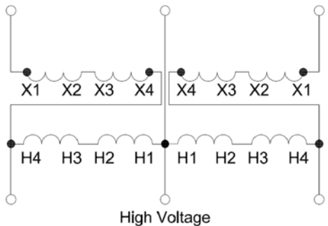
DIAGRAM "O"
