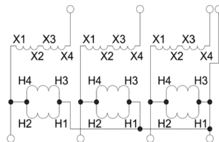
DIAGRAM "N"
