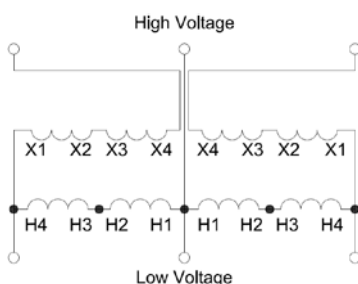
DIAGRAM “K”
