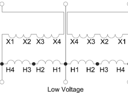
DIAGRAM "N"
