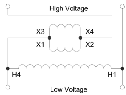
DIAGRAM "U"
