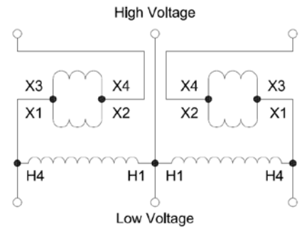
DIAGRAM "T"
