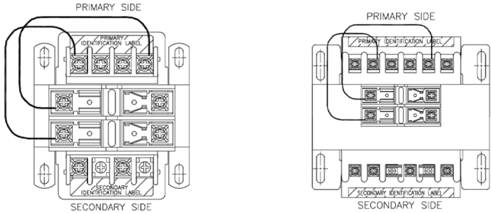
DIAGRAMS BELOW DEPICT NON-SERIES 2 PRIMARY FUSING OPTION
