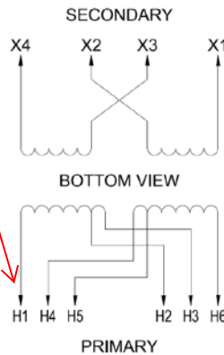
DIAGRAM "D"
