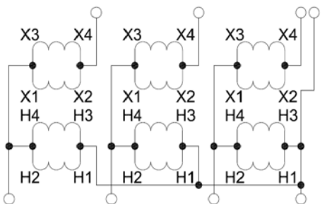
DIAGRAM "M"
