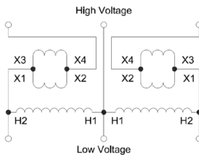
DIAGRAM "J"
