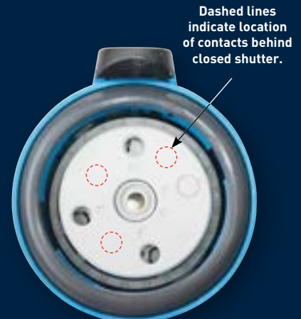
MELTRIC receptacle safety shutters minimize access to live contacts.
