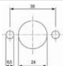
Mounting Diagram
