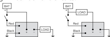
High side switching application Low side switching application
