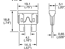
Dimensions inches [mm]
