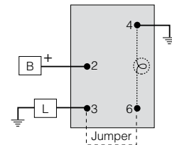
SPST Off-Off - Independent converted to Dependent (Four terminals) Connect jumper wire from T3 to T6 and connect T4 to ground Diagram G2
