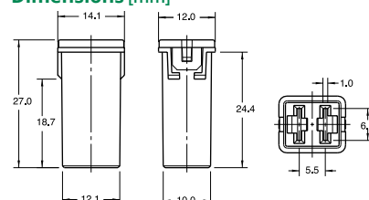
Dimensions [mm]
