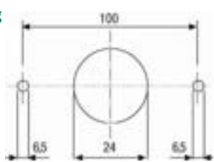
Mounting Diagram
