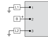
SPDT On-Off-On (3 terminals) Diagram B
