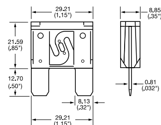
Dimensions inches [mm]
