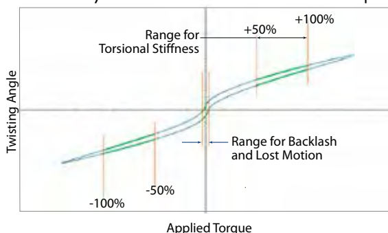
Gearbox Hysteresis Curve for \pm 100\% Nominal Torque
