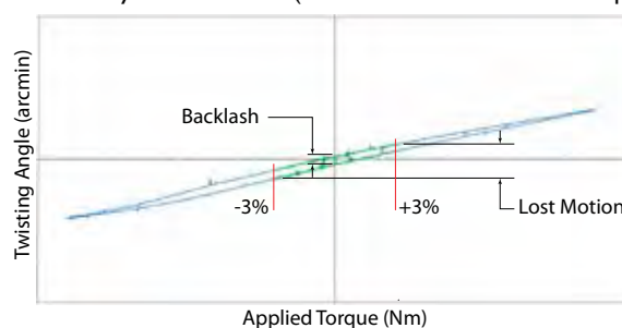
Gearbox Hysteresis Curve (detail of \pm 3\% of Nominal Torque)
