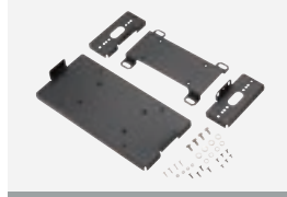
IPX-LPV2 Adjustable license plate bracket, mounts MPS3U/MPS6U/MPS12U lights to the license plate of popular vehicles
