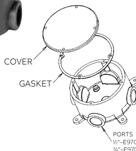
Conduit bodies Type X with cover
