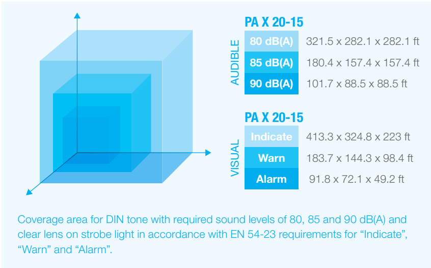
3D-Coverage Performance Data, A x B x C
