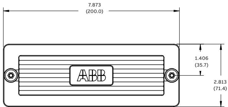
— 41 FT-14 shallow cover
