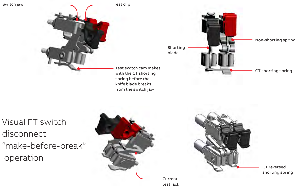
Blade assembly of two-position current poles
