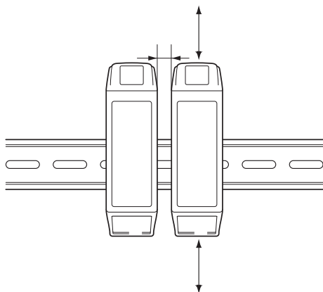
Figure 7. Minimum spacing of product
