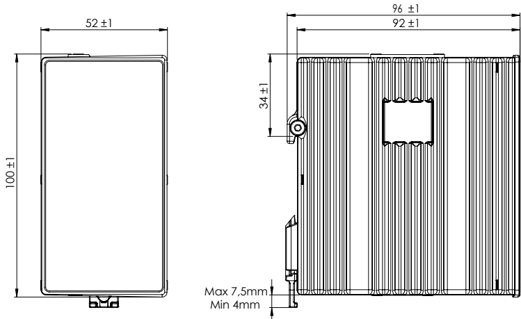
Figure 6. Dimensional drawing
