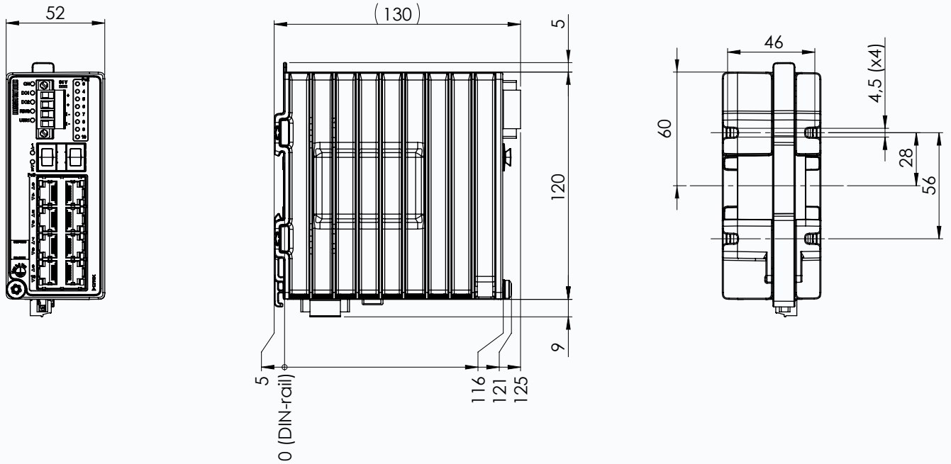
Dimensional drawing
