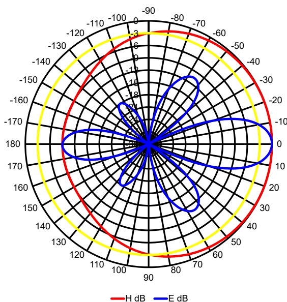
RADIATION PATTERN
