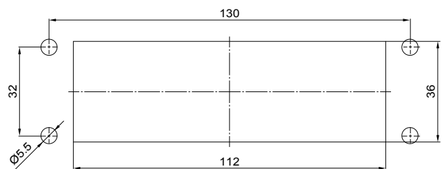
Hole Dimensions
