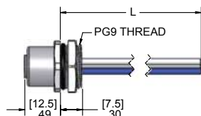
Female Receptacle
