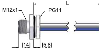
Male Receptacle
