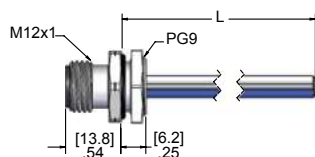
Male Receptacle
