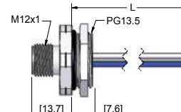
Male Receptacle
