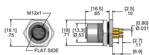
Female Receptacle
