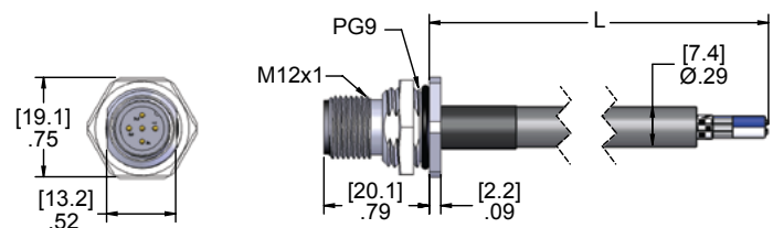
Male Receptacles
