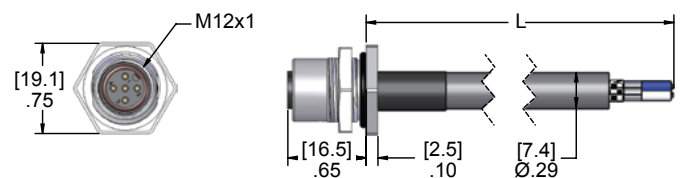
Female Receptacles
