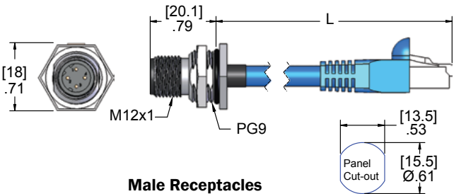
Male Receptacles
