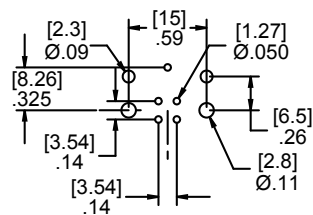
4 Pole Female Straight Layout
