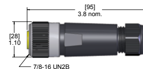
Female Straight (Female Threads)
