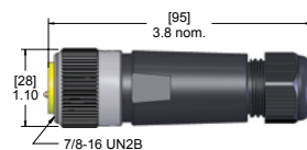
Male Straight (Female Threads)
