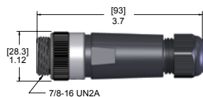
Male Straight (Male Threads)
