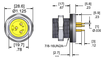
Male Back Mount Receptacle
