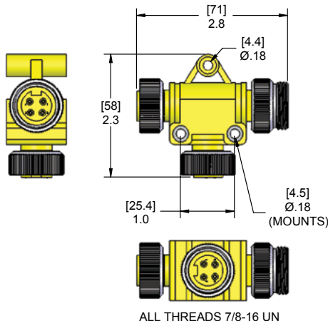
7/8”-16UN to 7/8”-16UN “T” Connector
