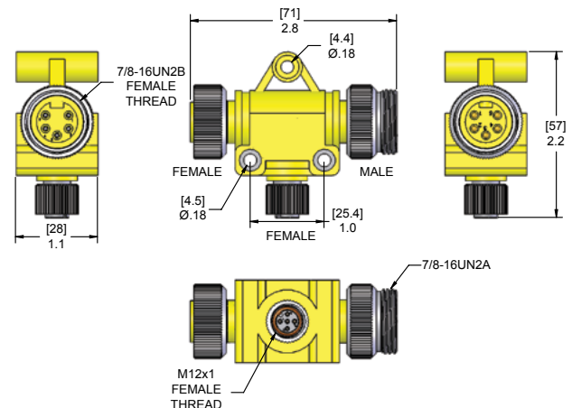
7/8”-16UN to M12 “T” Connector
