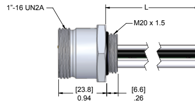
M20 Threads
