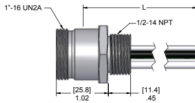
1/2"-14 NPT Threads
