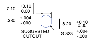
Male Receptacle
