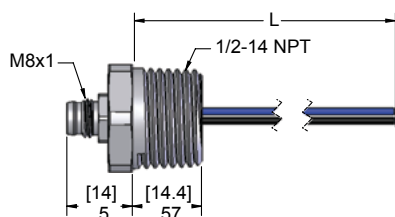
Male Receptacle
