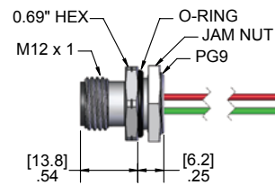
Male Receptacle
