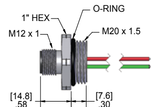
Male Receptacle
