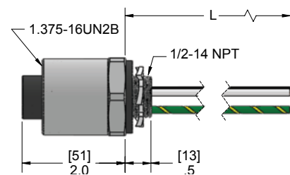
Female Receptacles
