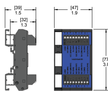
Spring Clamp Terminal Block to Spring Clamp Terminal Block with 3 Removable Marker Tags
