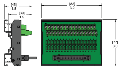
34 Pin Ribbon Cable to Terminal Block
