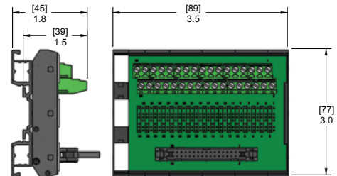
34 Pin Ribbon Cable to Terminal Block with 3 Removable Marker Tags
