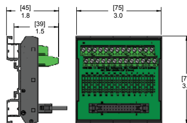
26 Pin Ribbon Cable to Terminal Block
