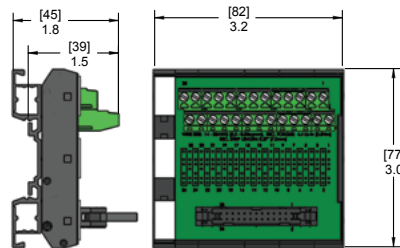
26 Pin Ribbon Cable to Terminal Block with 3 Removable Marker Tags
