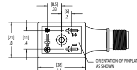
2 Poles + Ground (Ground Opposite Receptacle Side)
