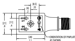
2 Poles + Ground (Ground Receptacle Side)
