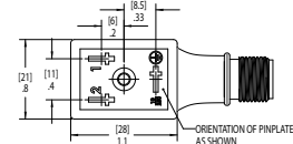
2 Poles + Ground (Ground Receptacle Side)
