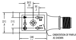
2 Poles + Ground (Ground Opposite Receptacle Side)
