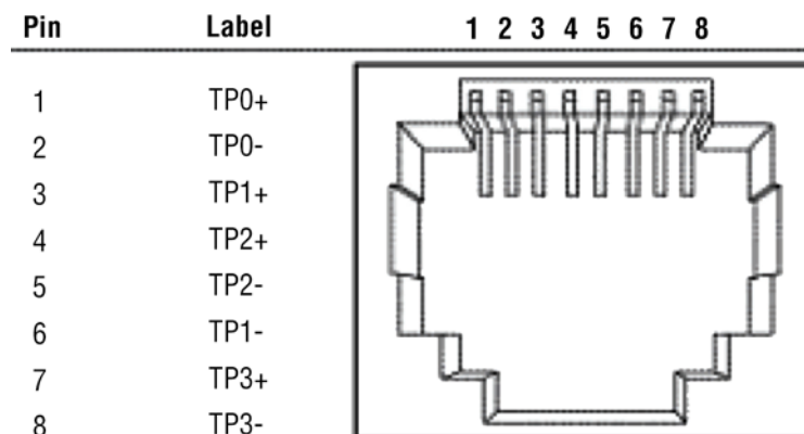
Figure 4. RJ-45 Ethernet port pin-outs
