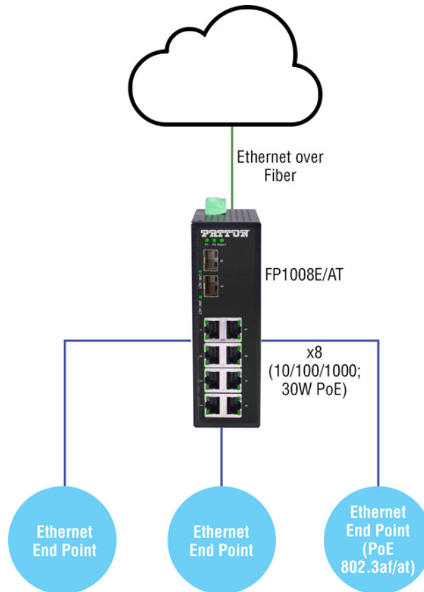
Figure 21. Industrial Ethernet Switch Application Reference
