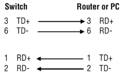
Figure 2. Straight-through cable schematic
