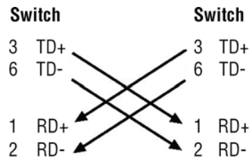
Figure 3. Crossover cable schematic
