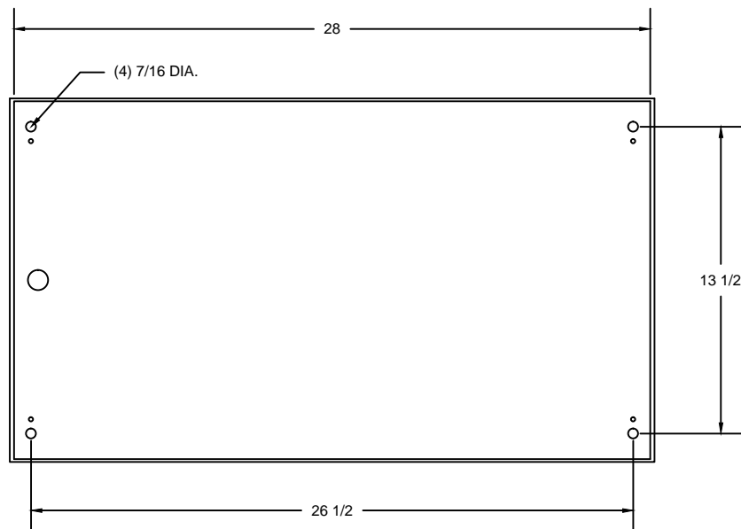
BOTTOM VIEW
