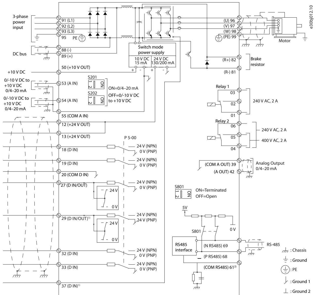
Illustration 5: Wiring Schematic
