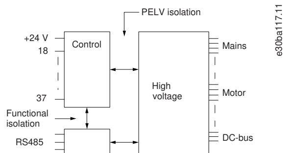
Illustration 12: PELV Isolation
