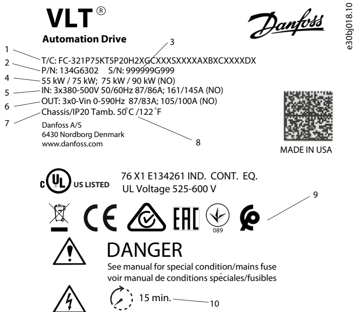
Illustration 1: Nameplate Example
