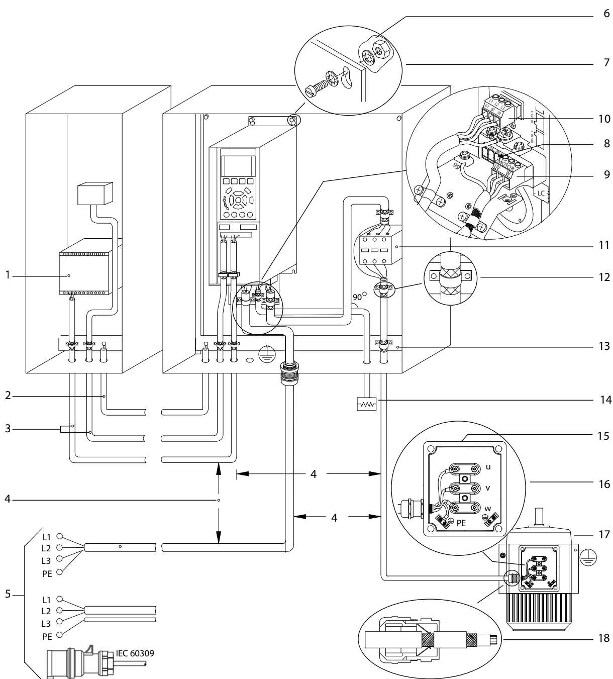
Illustration 4: Example of Proper EMC Installation
