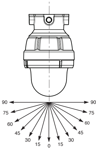
Model 24XSTHI Visible Signaling Device for the Hearing Impaired Light Dispersion Pattern per UL1971
