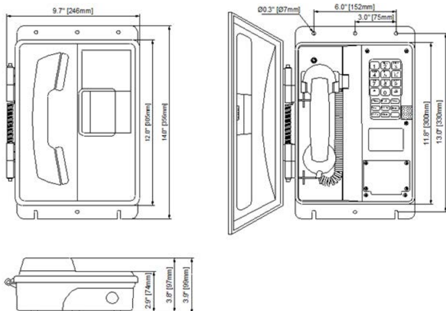
Figure 3 Dimensions
