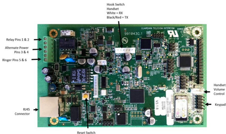
Figure 5 Circuit Board
