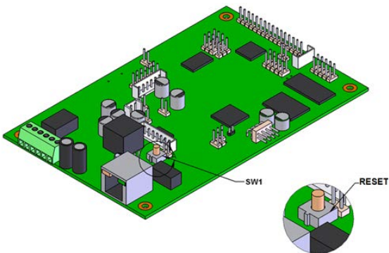
Figure 9 RESET Switch
