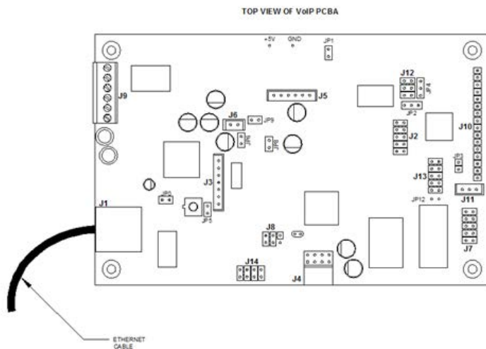
Figure 4 Wiring
