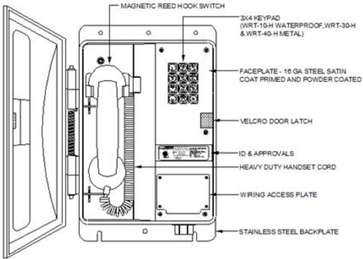
Figure 1 Features
