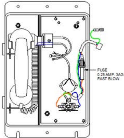
Figure 4 Fuse Replacement
