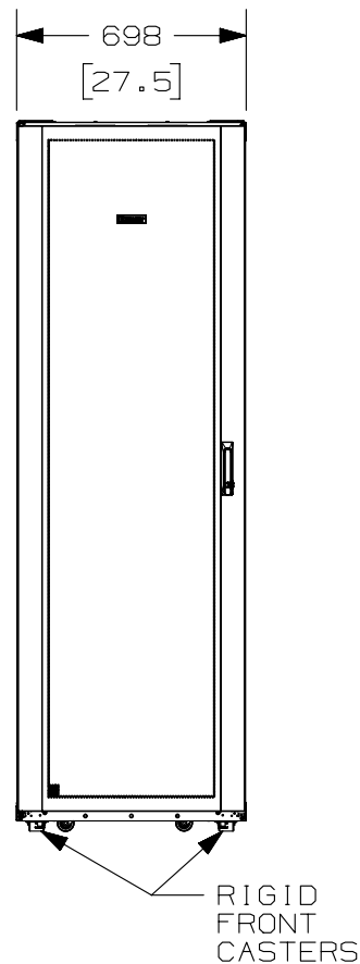
FRONT VIEW
