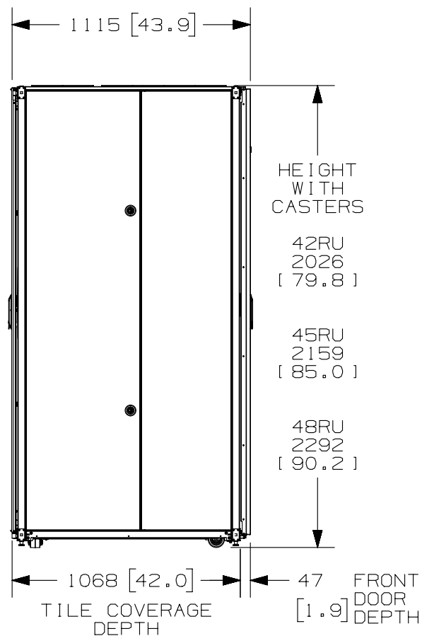
LEFT VIEW
