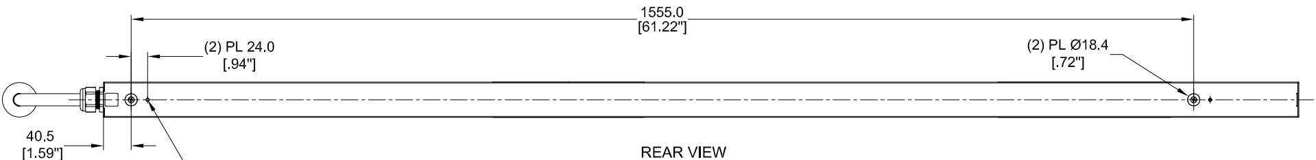
REAR VIEW
