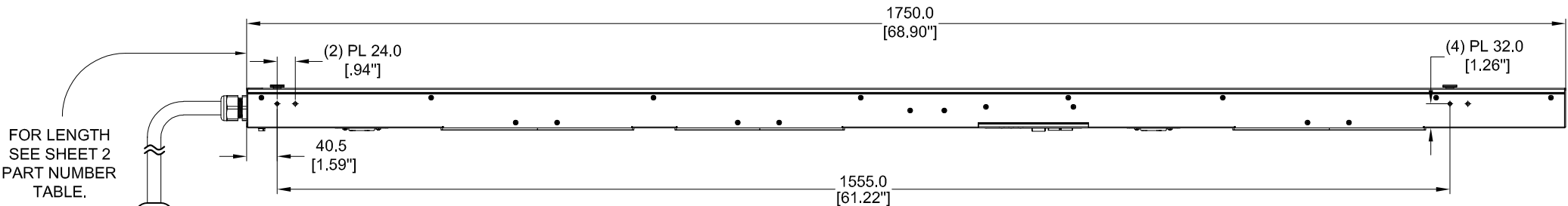
RIGHT VIEW
