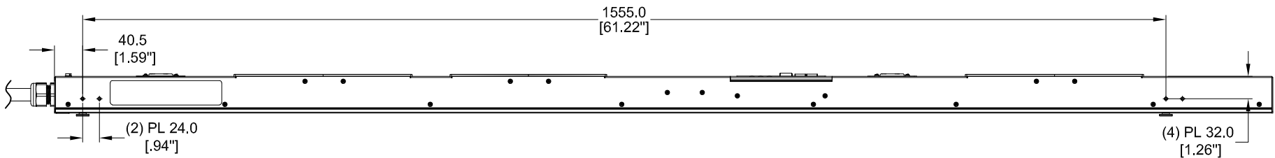
LEFT VIEW
