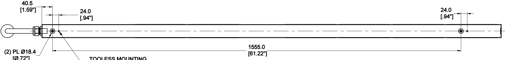
REAR VIEW
