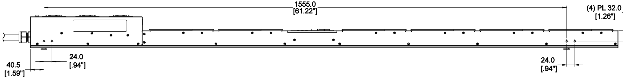
LEFT VIEW
