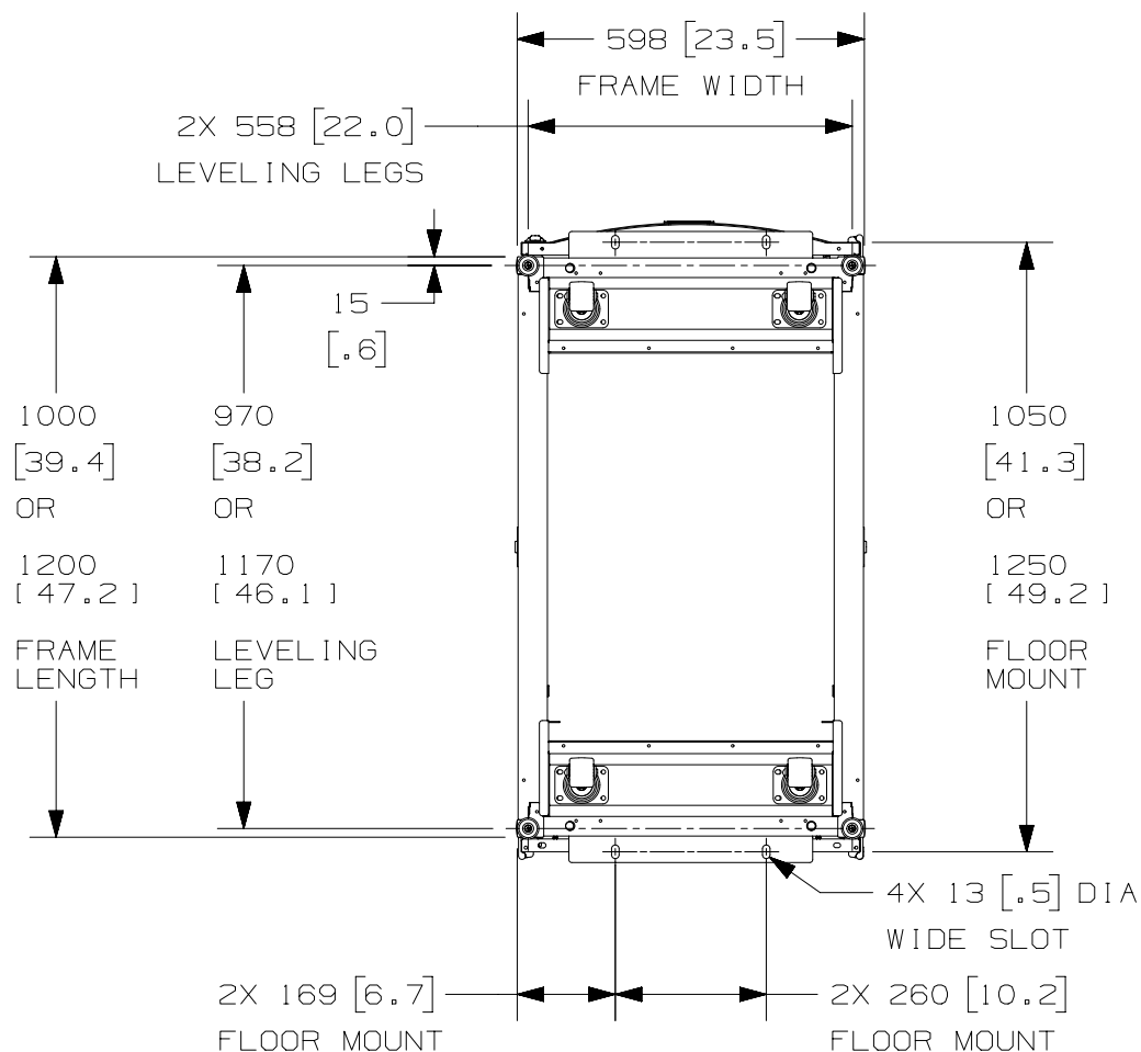
REAR OF CABINET BOTTOM VIEW
