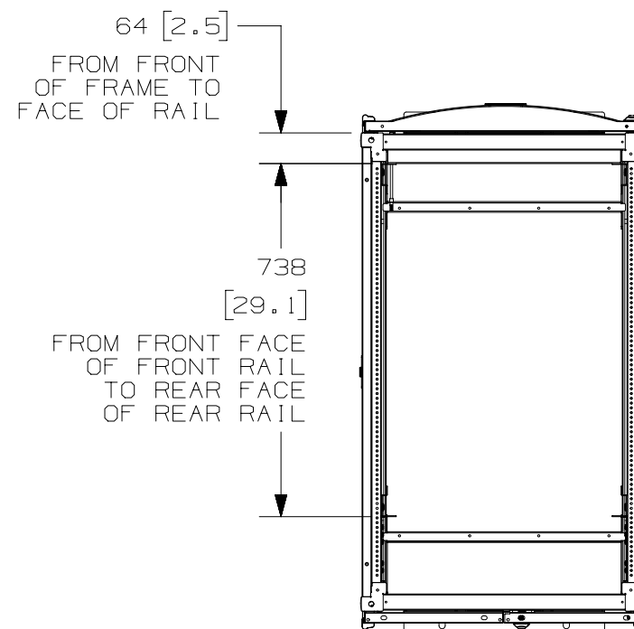
REAR OF CABINET TOP VIEW
