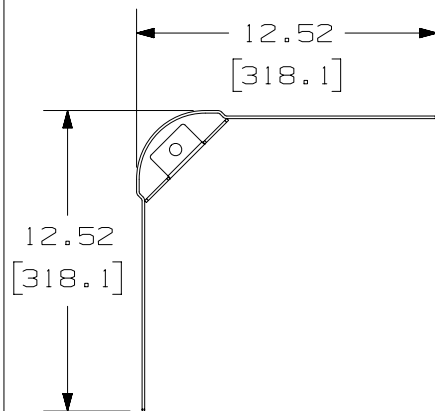
SUPPORT BRACKET
