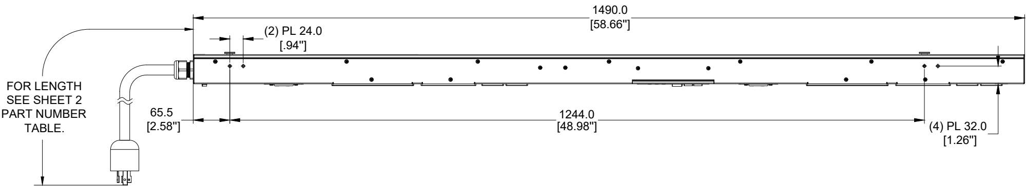
RIGHT VIEW
