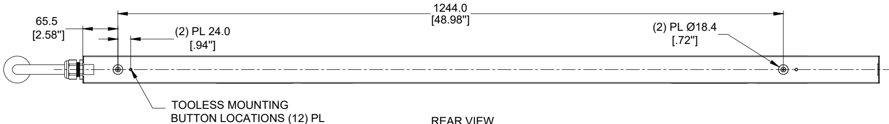
REAR VIEW
