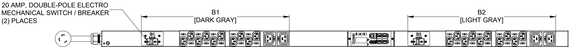
FRONT VIEW
