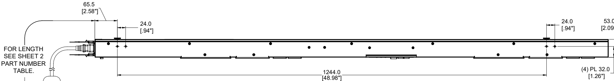
RIGHT VIEW
