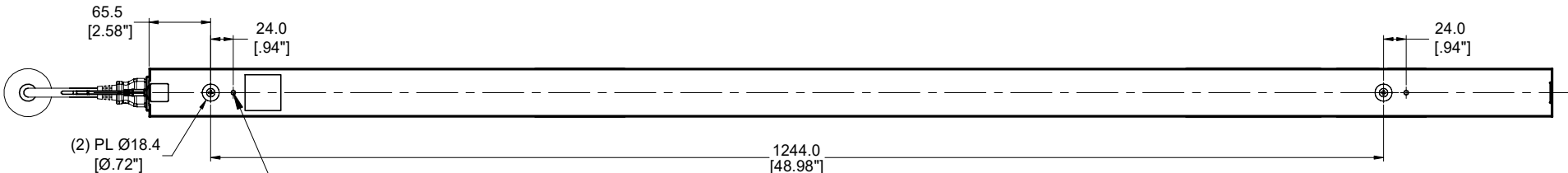
REAR VIEW
